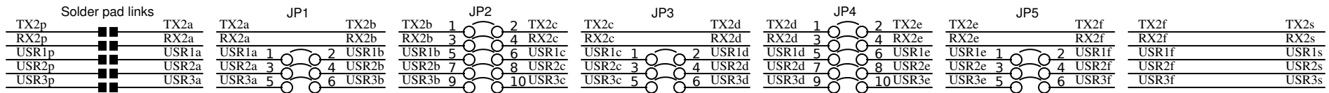
BP80 Section Plug p RC80 Card Socket a RC80 Card Socket b RC80 Card Socket c RC80 Card Socket d RC80 Card Socket e RC80 Card Socket f BP80 Section Socket s
